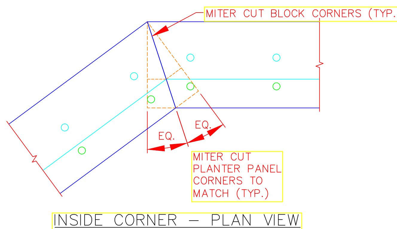
G MITERED CORNER JOINT DETAIL 1-1/2" = 1'-0"
