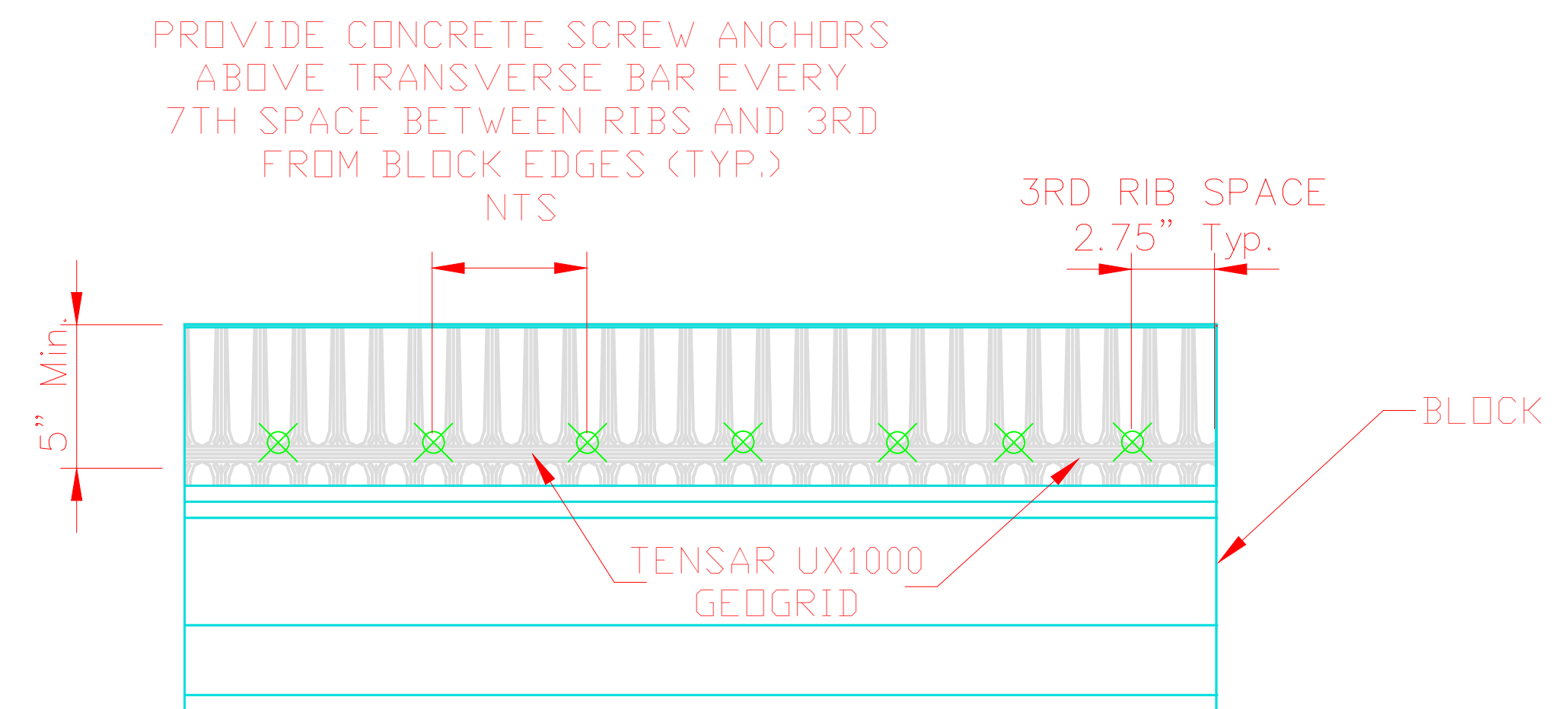
C SECONDARY GEOGRID CONNECTION TO BLOCK N.T.S.
