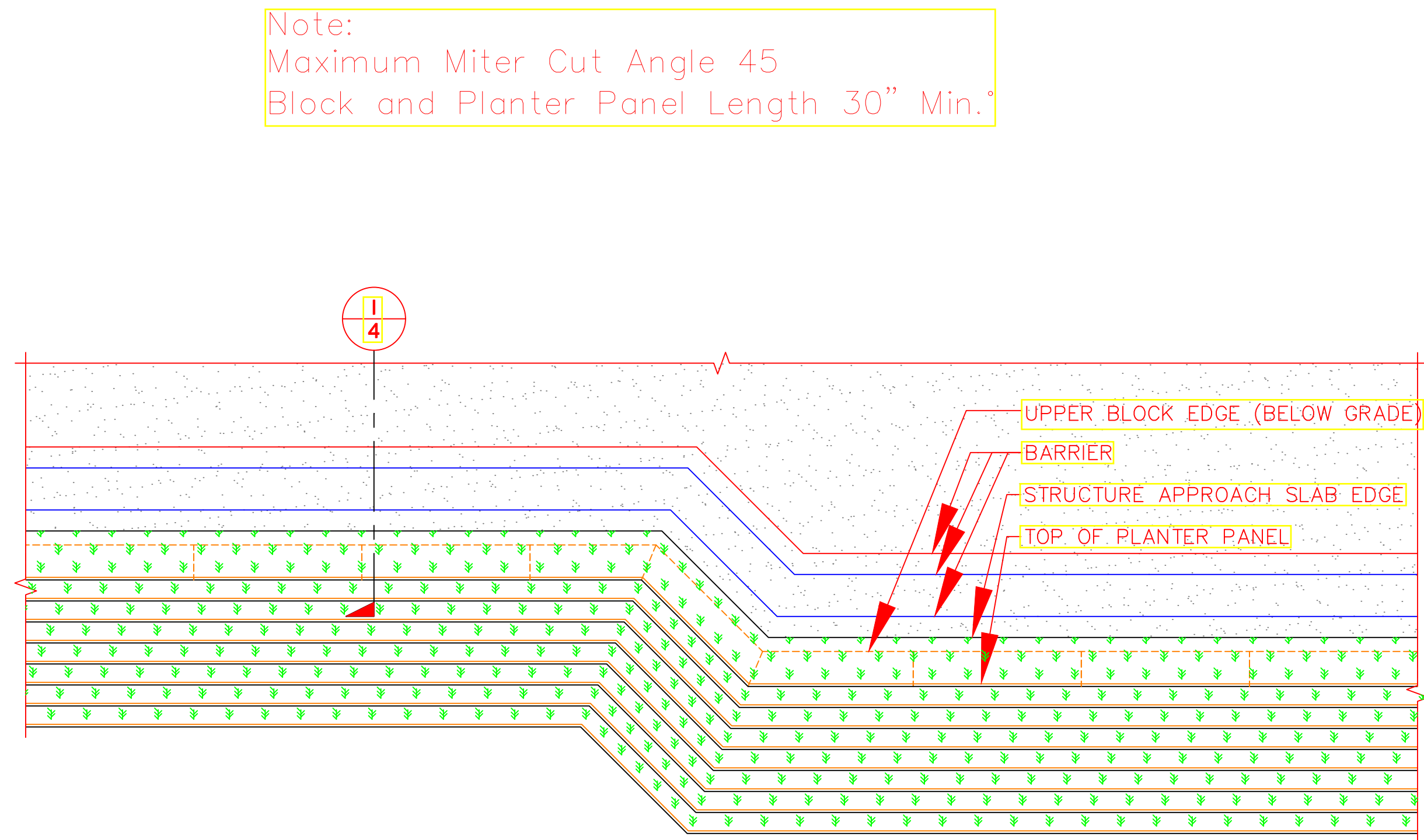
H PLAN VIEW 3/8" = 1'-0"
