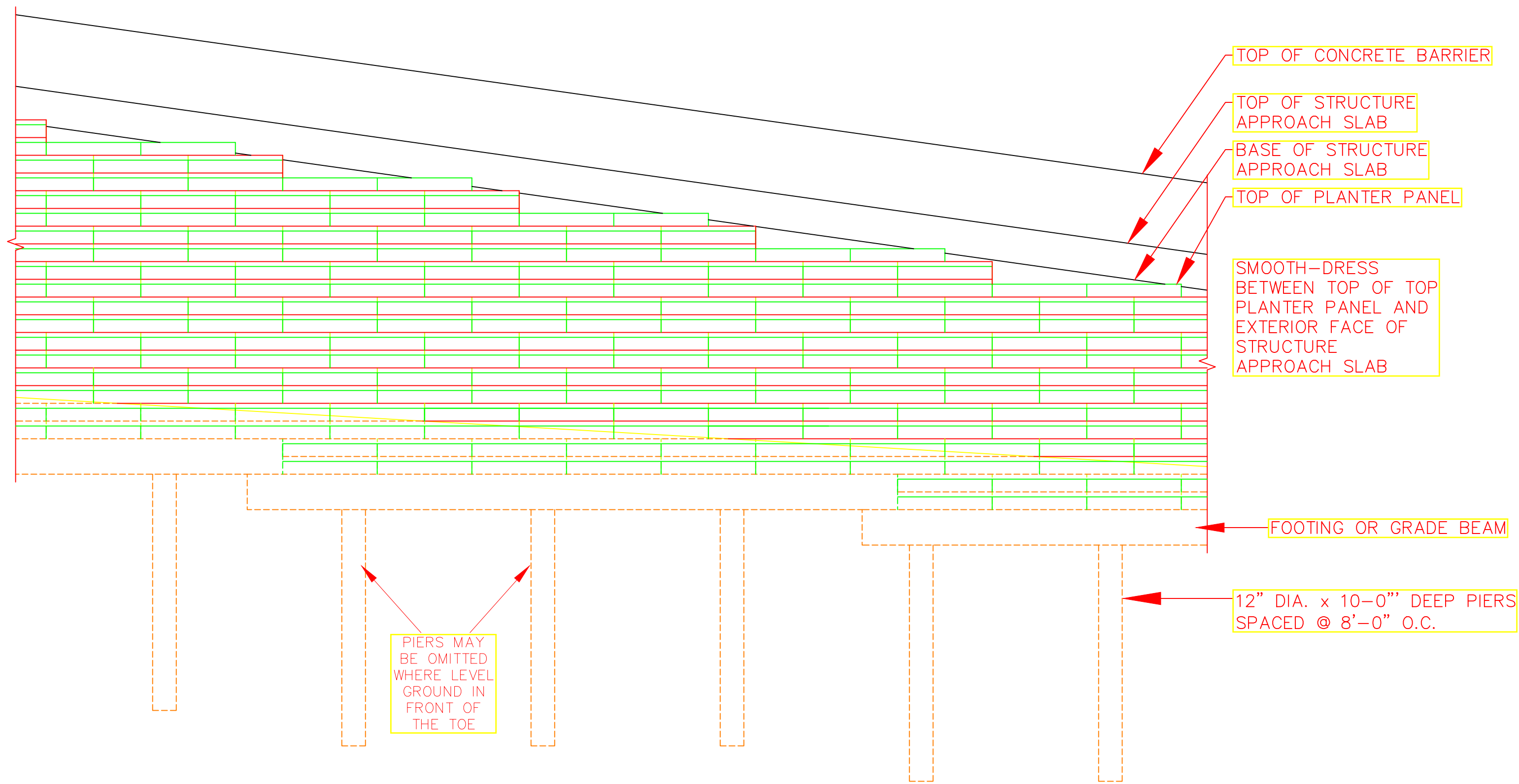
F FRONT ELEVATION VIEW 1/4" = 1'-0"
